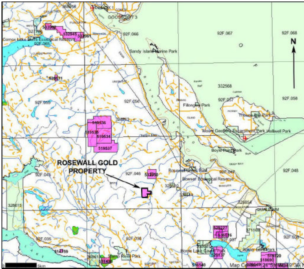
Fig. 2 ROSEWALL GOLD PROPERTY REGIONAL LOCATION MAP 6
