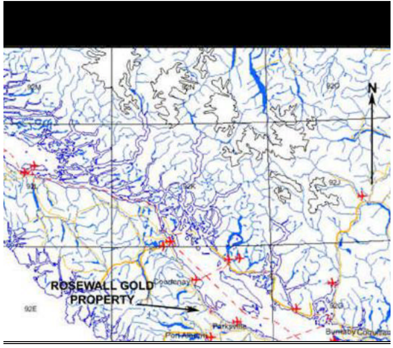
Fig. 1 ROSEWALL GOLD PROPERTY BC LOCATION MAP 5
