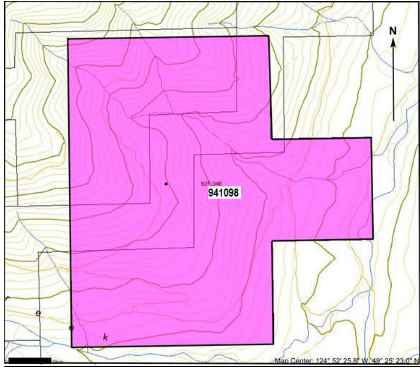
Fig. 3 ROSEWALL GOLD PROPERTY MAP 7
