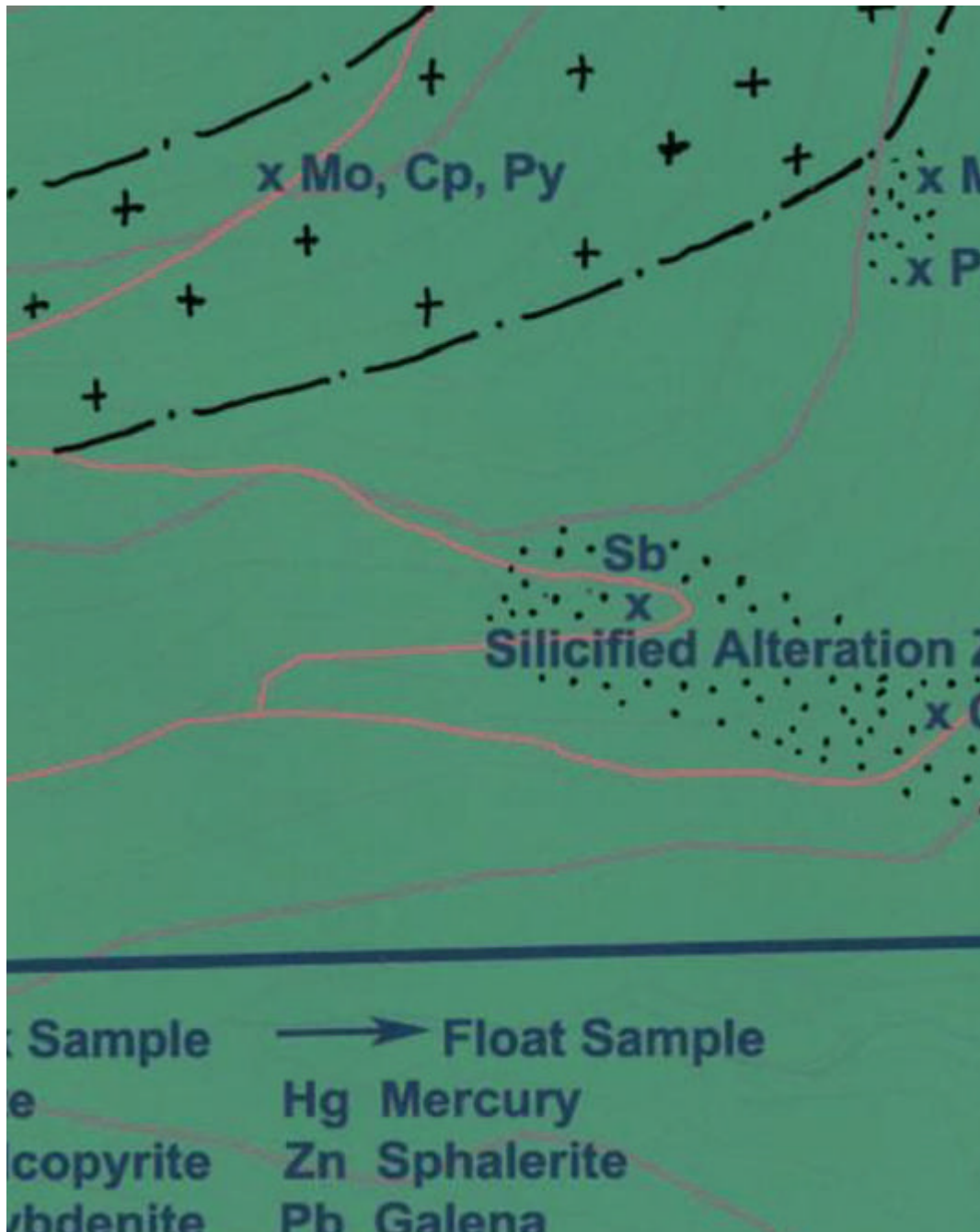
Fig. 4 REGIONAL GEOLOGY OF THE ROSEWALL GOLD PROPERTY 9
