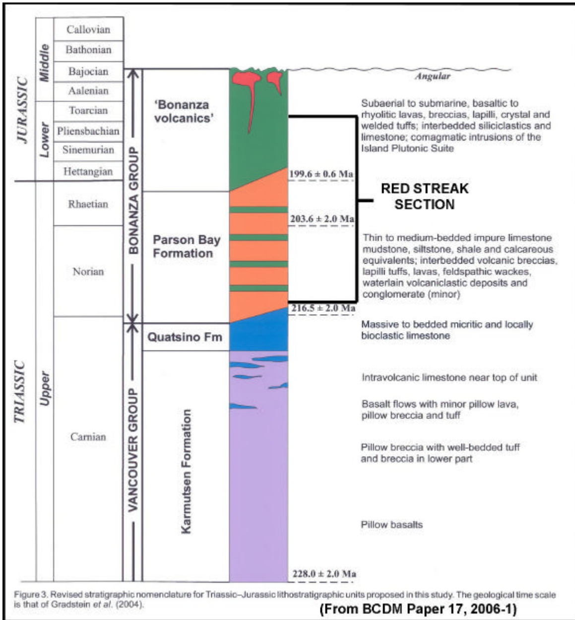
Fig. 5 RED STREAK AREA STRATIGRAPHIC COLUMN
