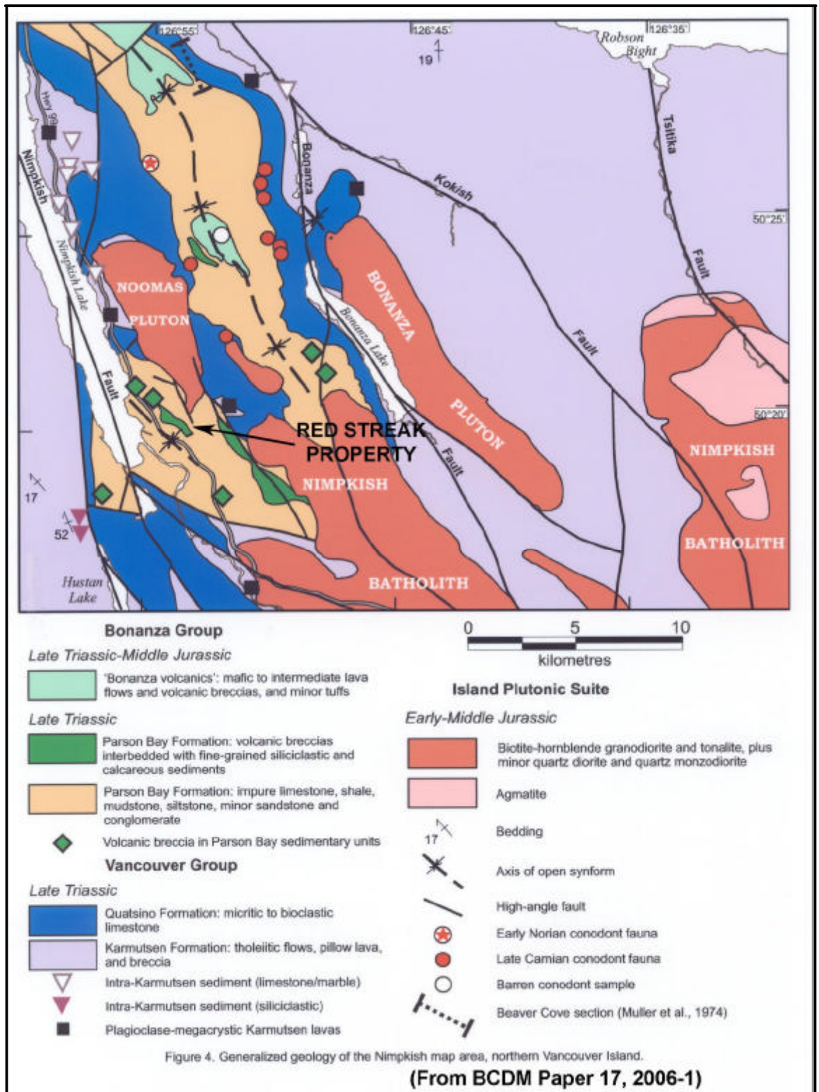
Fig. 4 NIMPKISH AREA GEOLOGICAL MAP
